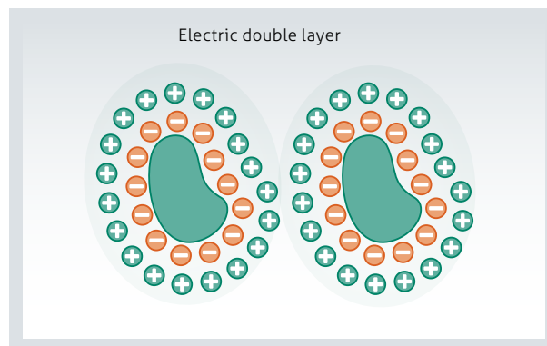
Figure 5 | Electrostatic stabilization
